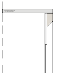
Maniglia Stone dx o sx Stone handle R or L
